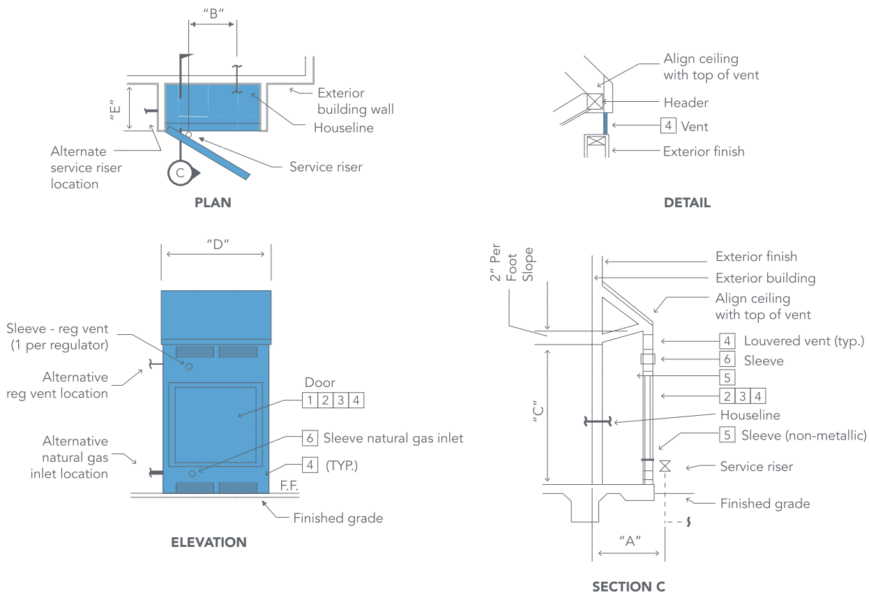
FIGURE 25 - Natural Gas Meter Enclosure – Single Meter Surface Mount
