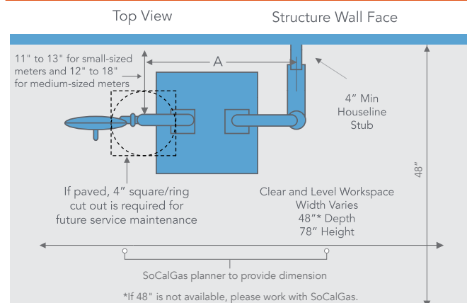
FIGURE 21 - Non-Residential Standard Delivery Natural Gas Meter Set - Top View
