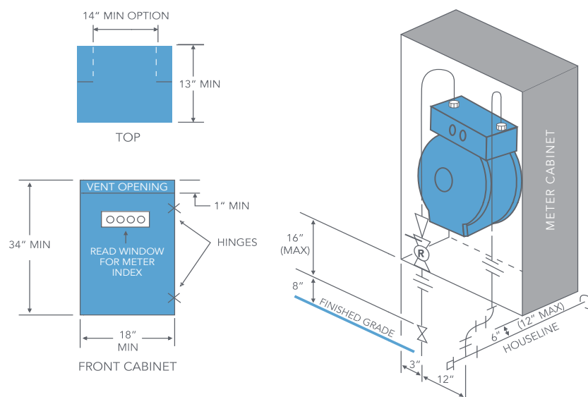
FIGURE 23 - Natural Gas Meter Cabinet Guidelines
