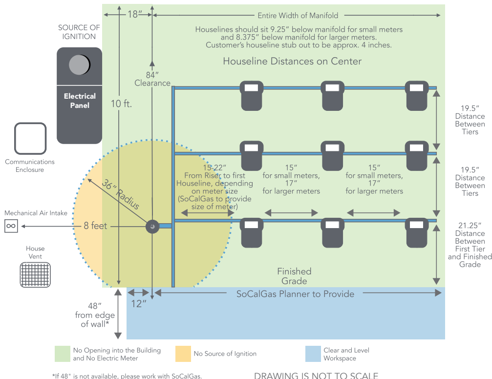
FIGURE 19C - Multi-family Three-Tier Natural Gas Meter Manifold
