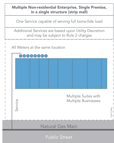
FIGURE 11 - Multiple Non-residential Enterprises on a Single Premise, Single Structure
