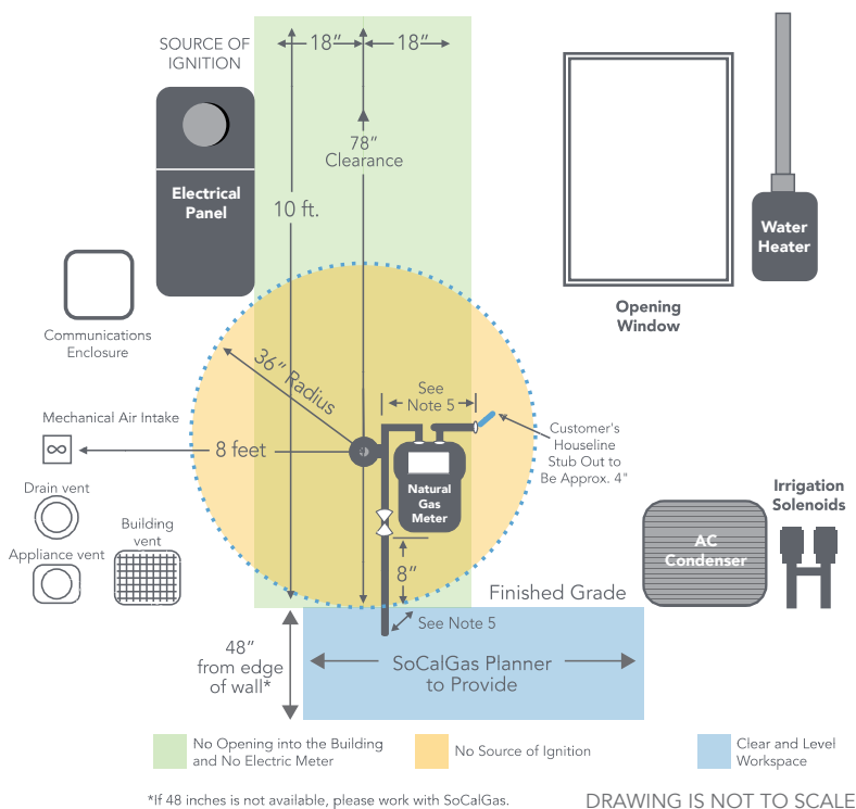
FIGURE 20 - New Non-Residential Natural Gas Meter Set Separation and Clearance Guidance Diagram
