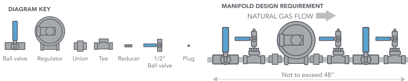
FIGURE 29 - Requirements for New Step-Down Manifolds for Non-Residential 2 PSIG, 5 PSIG and Above Systems
