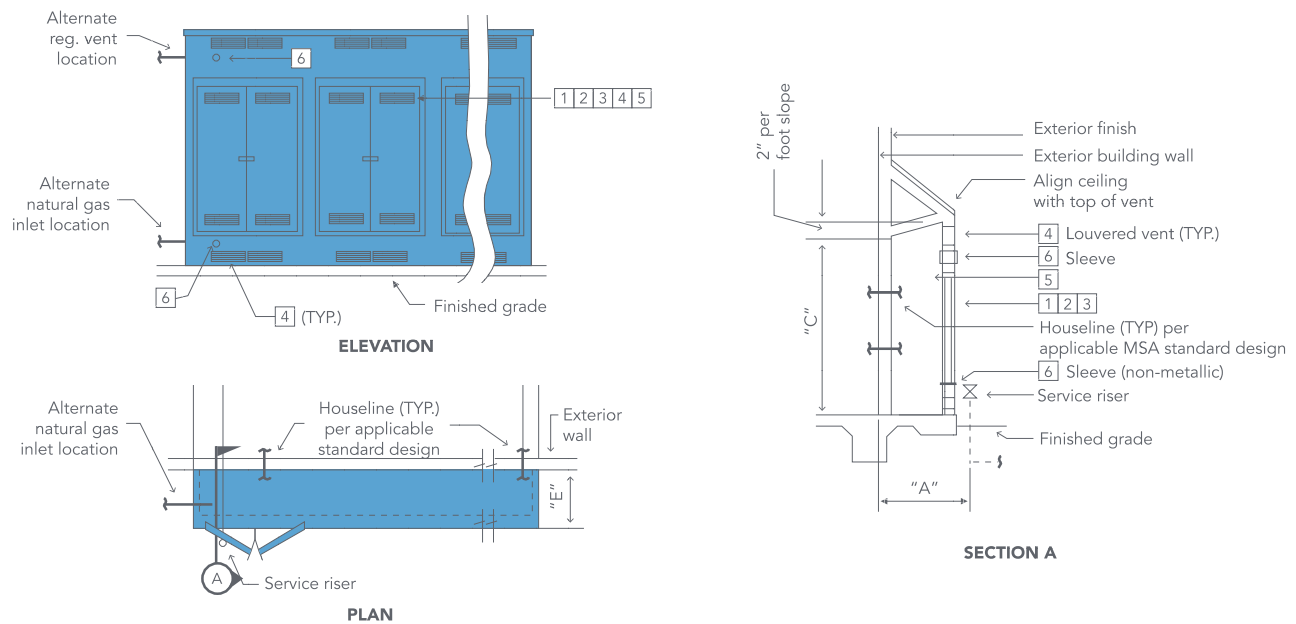
FIGURE 26 - Natural Gas Meter Enclosure – Multiple Meter Surface Mount
