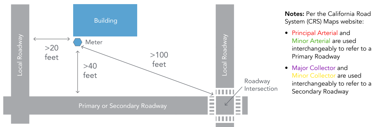
FIGURE 14 - Meter Locations — Distance from Roadways
