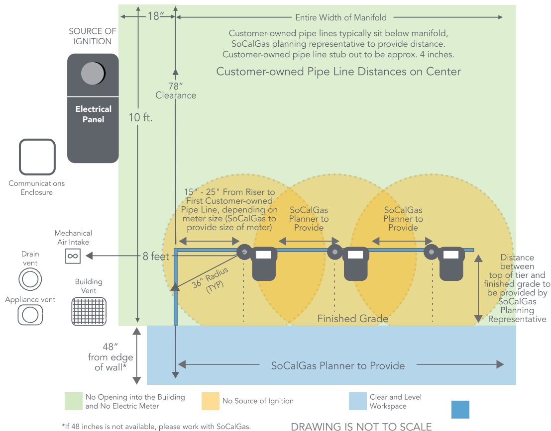
FIGURE 22 - Non-Residential Natural Gas Meter Manifold
