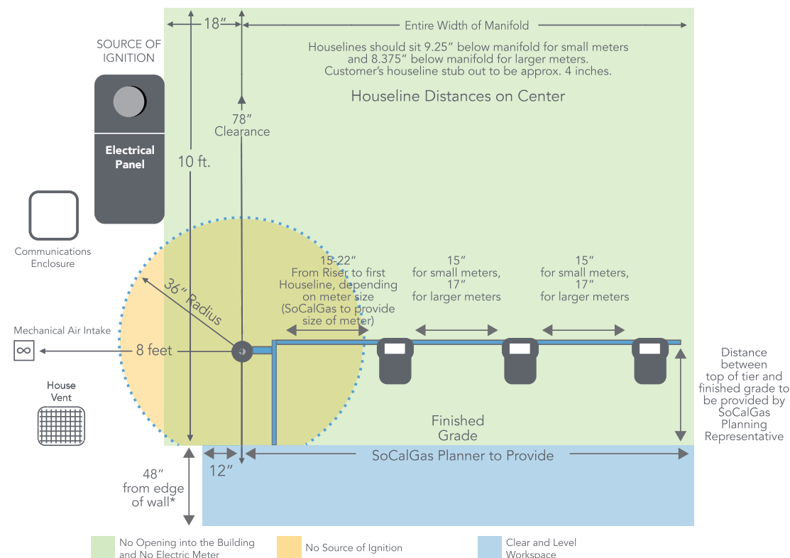
FIGURE 19A - Multi-family One-Tier Natural Gas Meter Manifold
