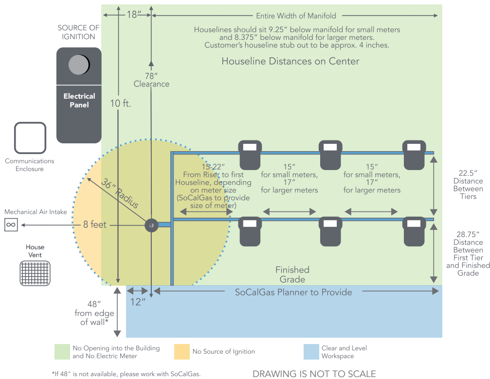
FIGURE 19B - Multi-family Two-Tier Natural Gas Meter Manifold
