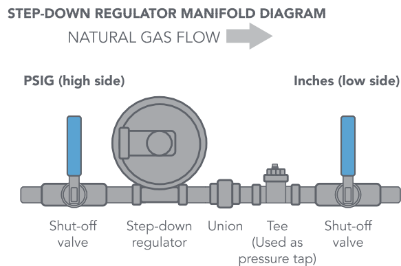
FIGURE 30 - Requirements for New Step-Down Manifolds for Residential 2 PSIG and 5 PSIG Systems
