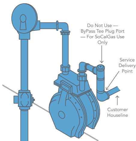
FIGURE 28 - Natural Gas Meter Service Delivery Point
