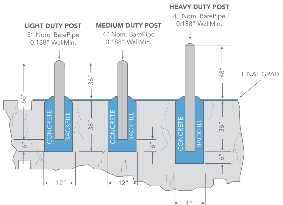
FIGURE 16 - Offset and Spacing of Protection Posts
