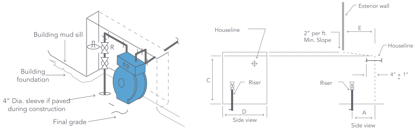
FIGURE 25 - Natural Gas Meter Enclosure – Single Meter Surface Mount
