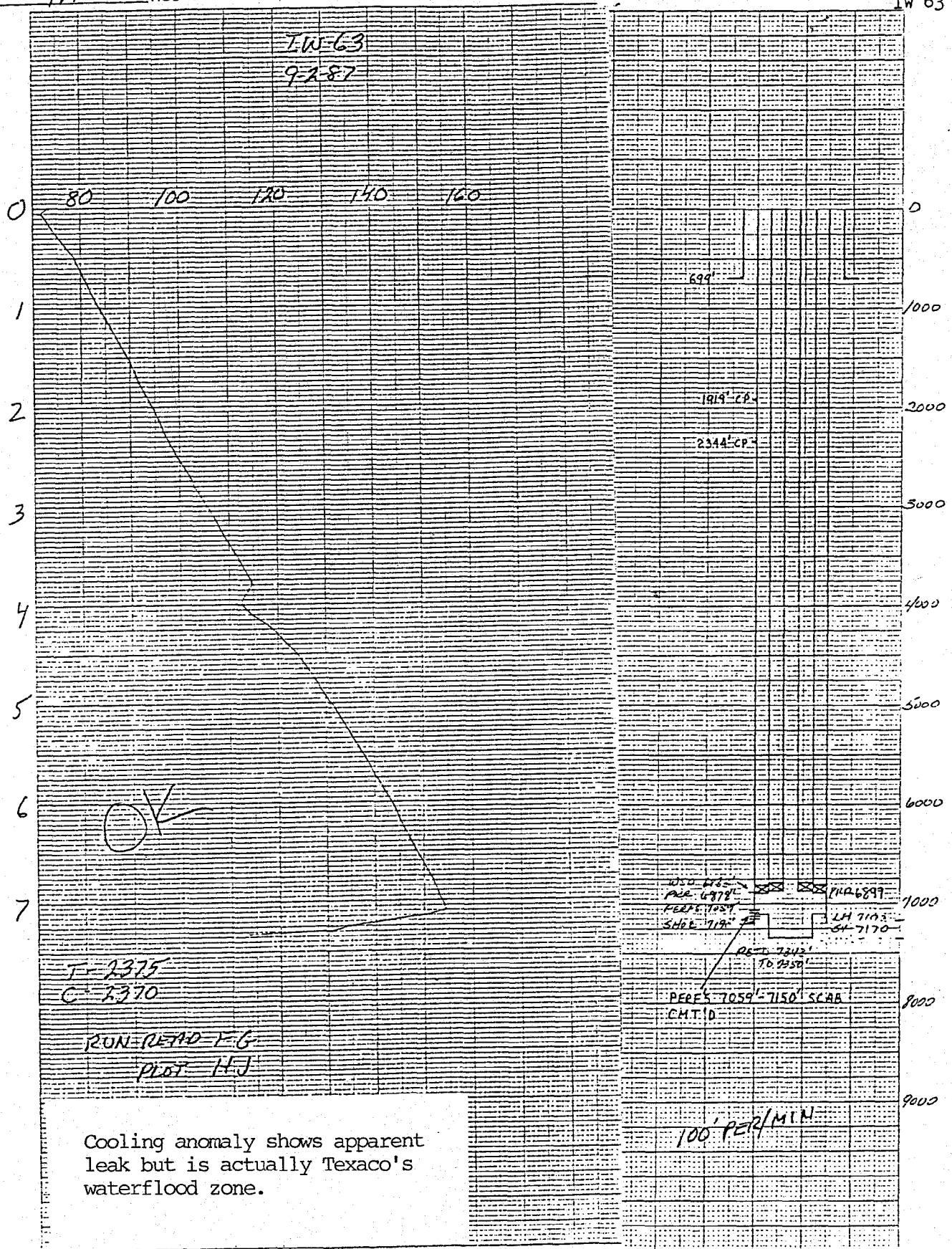
FIGURE 13. TEMPERATURE SURVEY
